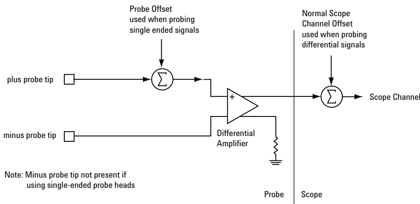
Figure 1. InfiniiMax Probe
